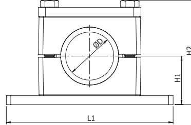
Çift Plakalı Montaj Delikli Kelepçe Double Plated Clamp with Elongated Weld Plate
